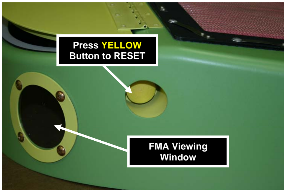
Figure 2-1. FILTER MAINTENANCE AID – (ABOVE) “YELLOW Indicator” position relative to SAFE OPERATING ZONE (“GREEN Zone”) or SERVICE FILTER (“RED Zone”) markings defines current filter condition and pushing “YELLOW RESET Button” resets indicator. (BELOW) FMA unit is mounted to inner frame of IBF assembly and can be viewed through access window in the upper fairing.
