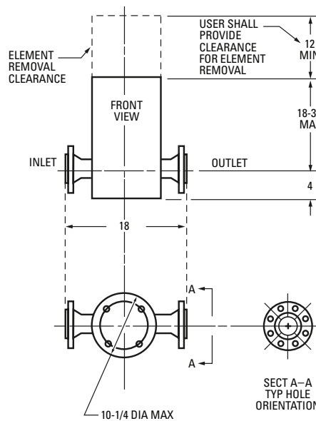
THREE-ELEMENT FILTER HOUSING OUTLINE DIMENSIONS
